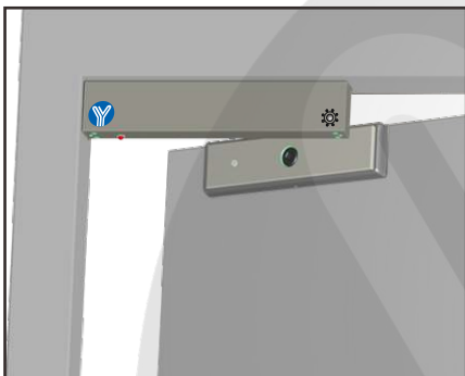
Demonstration of I Bracket Installation
