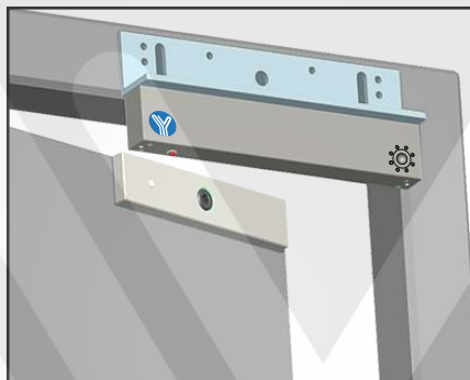
Demonstration of L Bracket Installation
