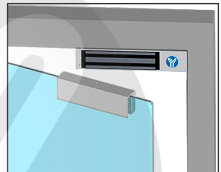
Demonstration of UL Bracket Installation
